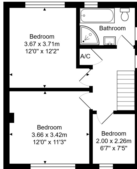
First Floor Area: 40.6 m 2 ... 437 ft 2
